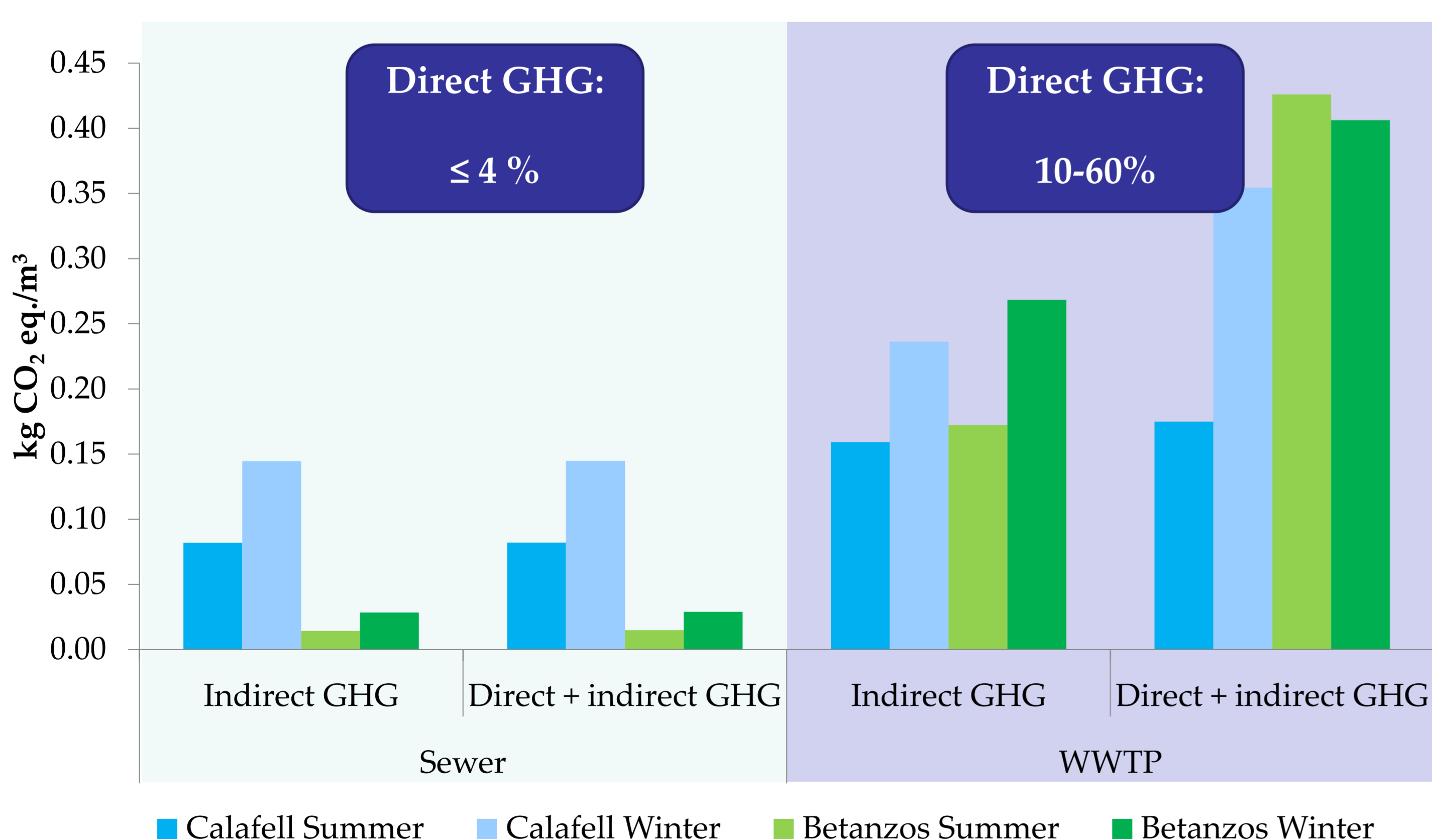
Figure 3. Integration of direct and indirect GHG emissions of the operation of sewers and WWTPs
